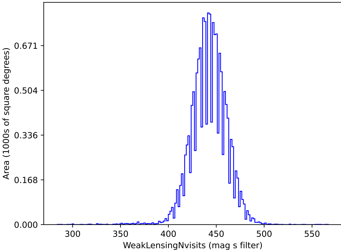
baseline_v2.0_10yrs gri band non-DD: WeakLensingNvisits
