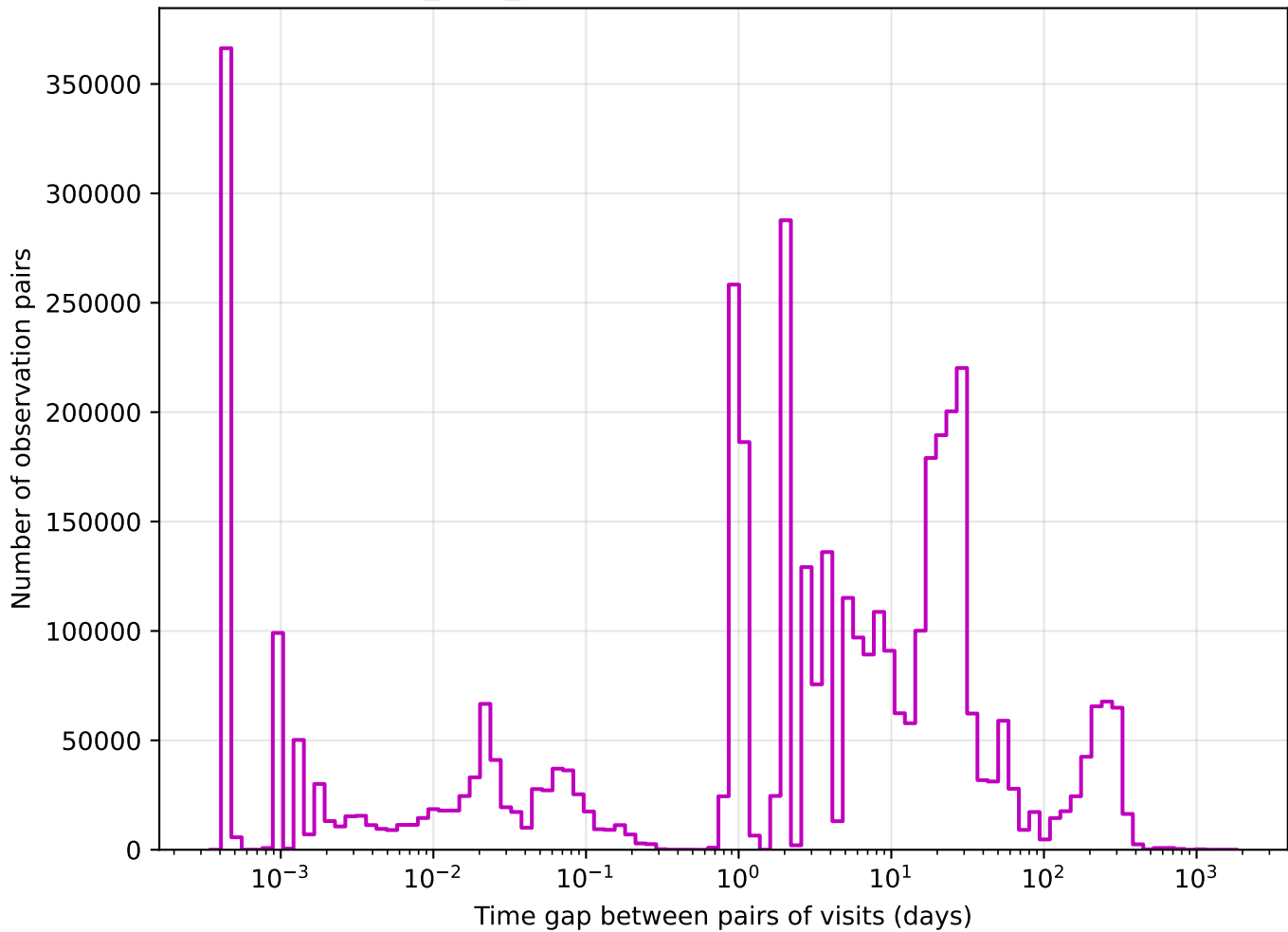
baseline_v2.0_10yrs z band: Tgaps observationStartMJD
