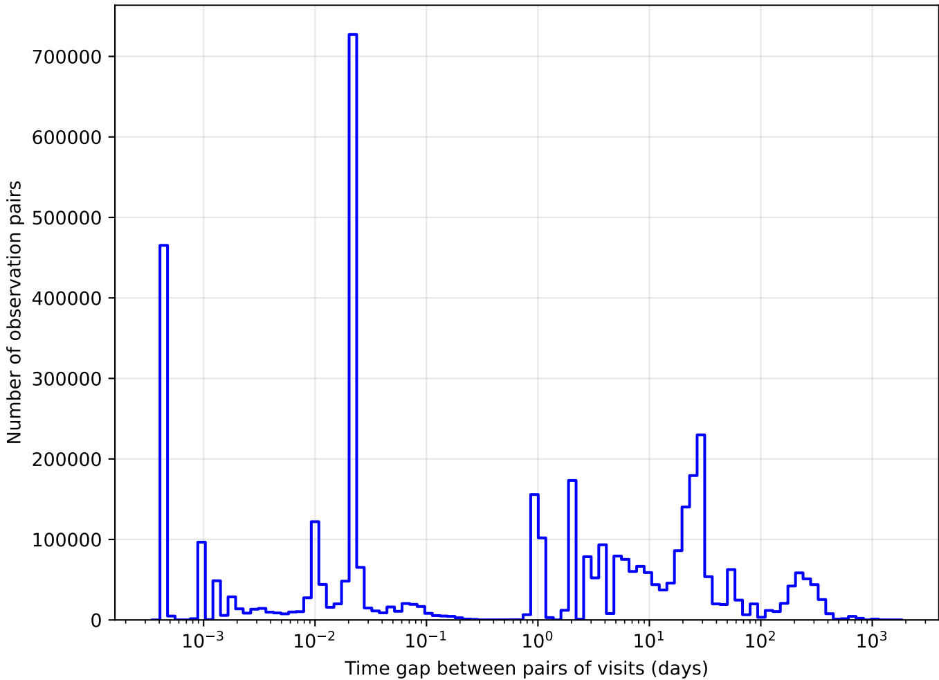
baseline_v2.0_10yrs y band: Tgaps observationStartMJD
