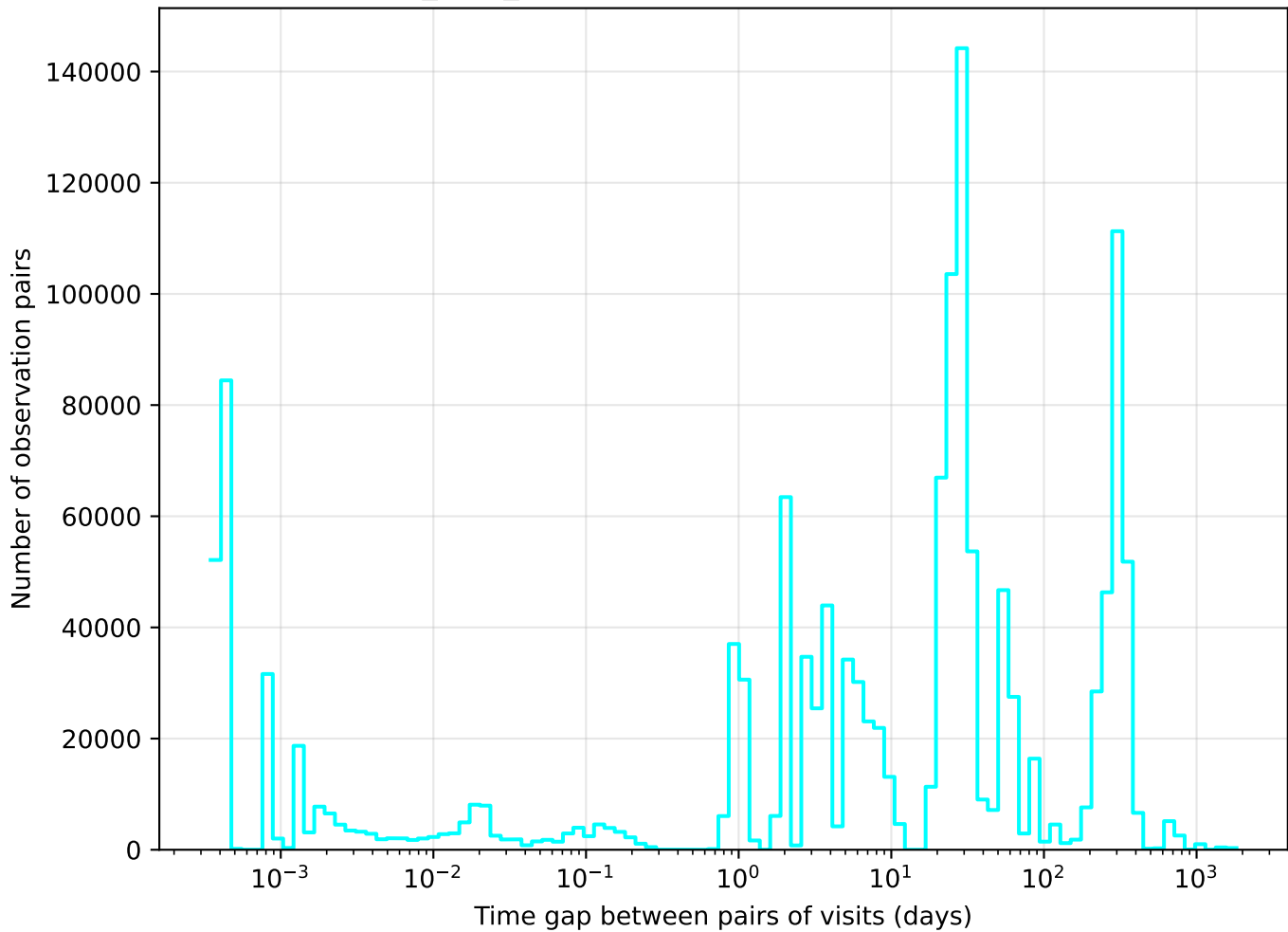
baseline_v2.0_10yrs u band: Tgaps observationStartMJD
