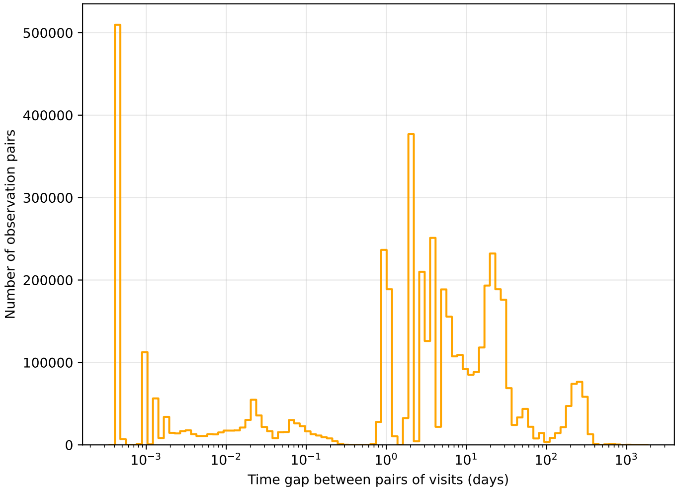
baseline_v2.0_10yrs r band: Tgaps observationStartMJD
