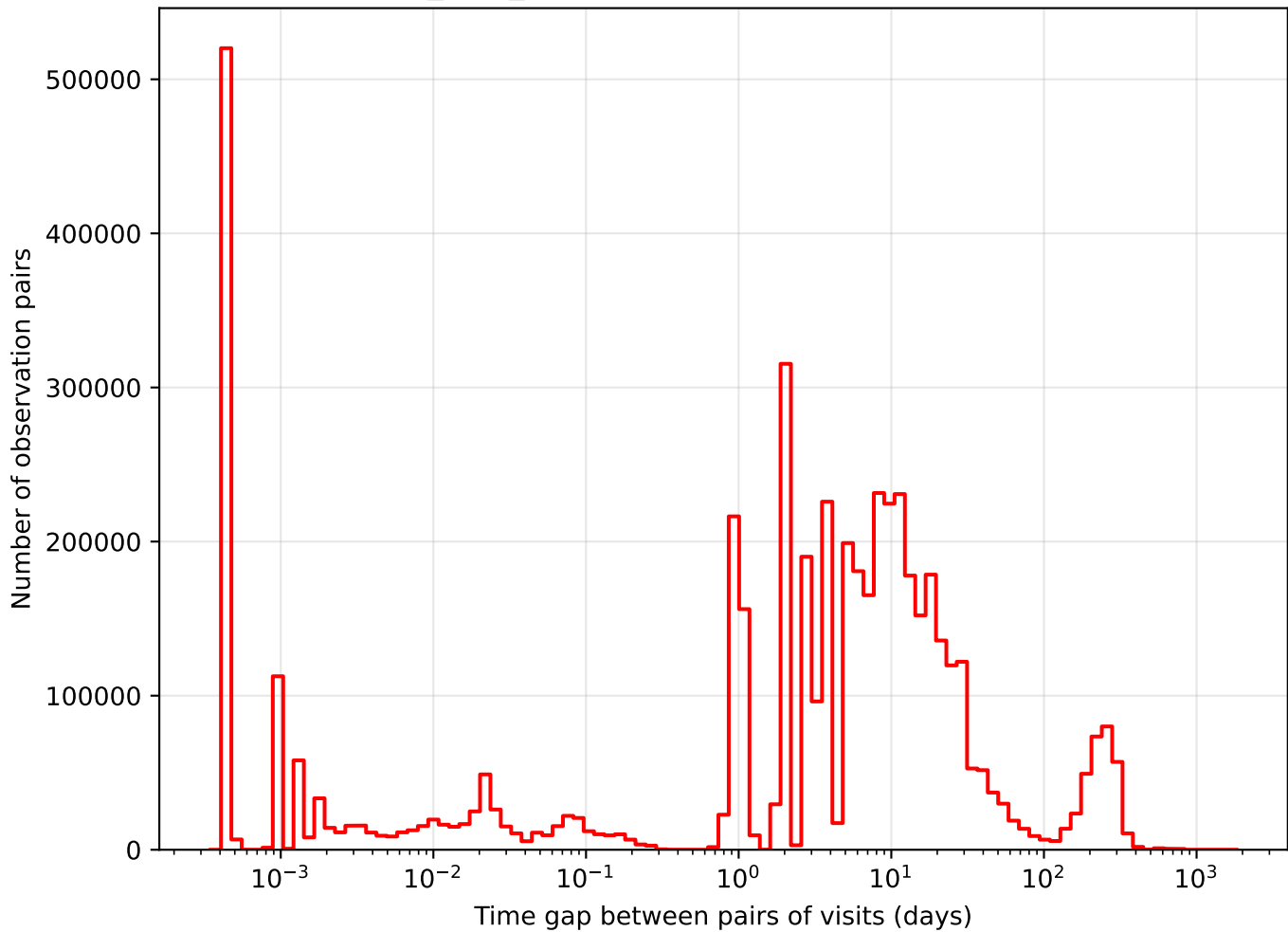
baseline_v2.0_10yrs i band: Tgaps observationStartMJD
