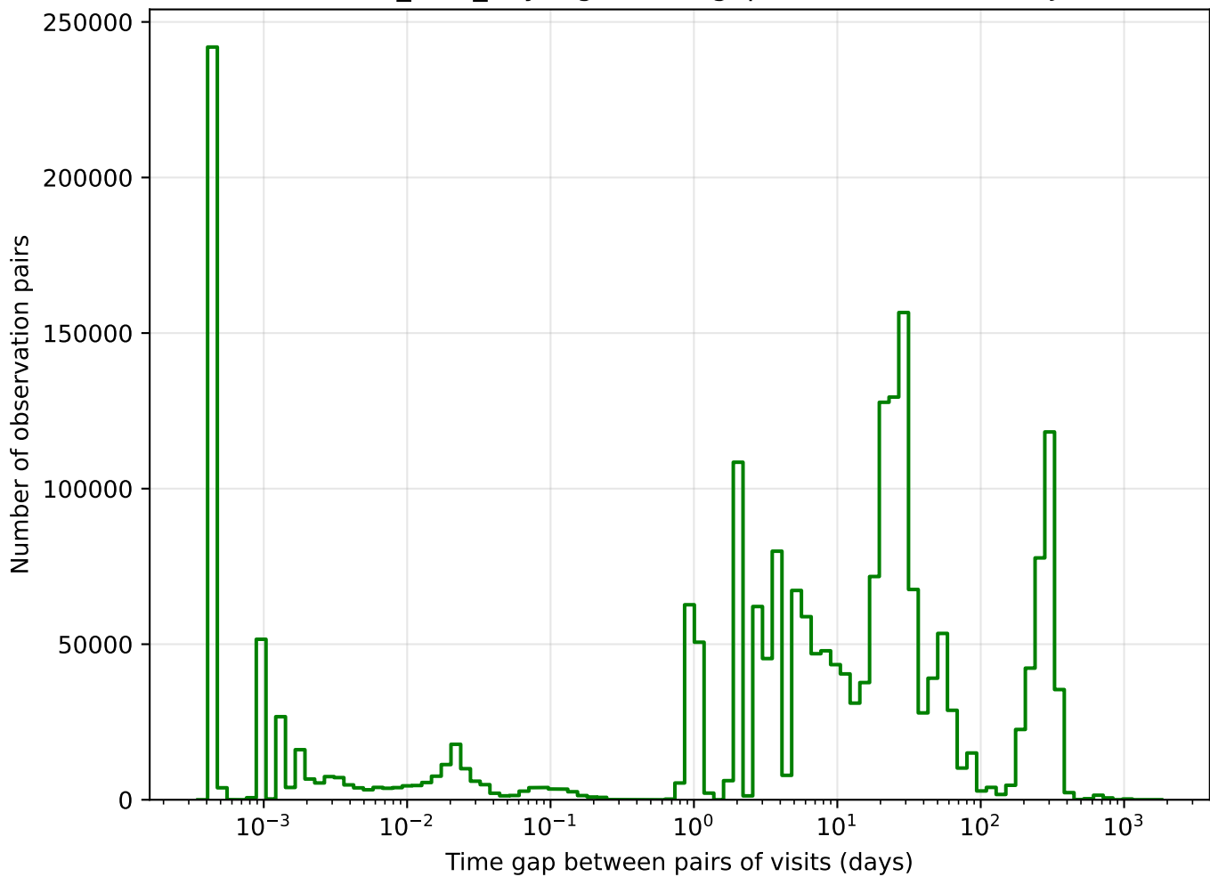
baseline_v2.0_10yrs g band: Tgaps observationStartMJD
