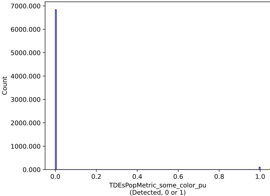
baseline_v2.0_10yrs : TDEsPopMetric_some_color_pu
