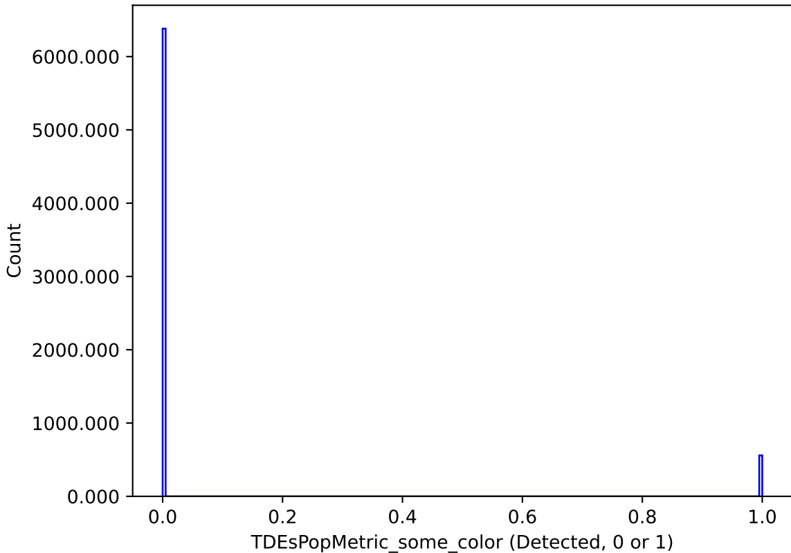
baseline_v2.0_10yrs : TDEsPopMetric_some_color
