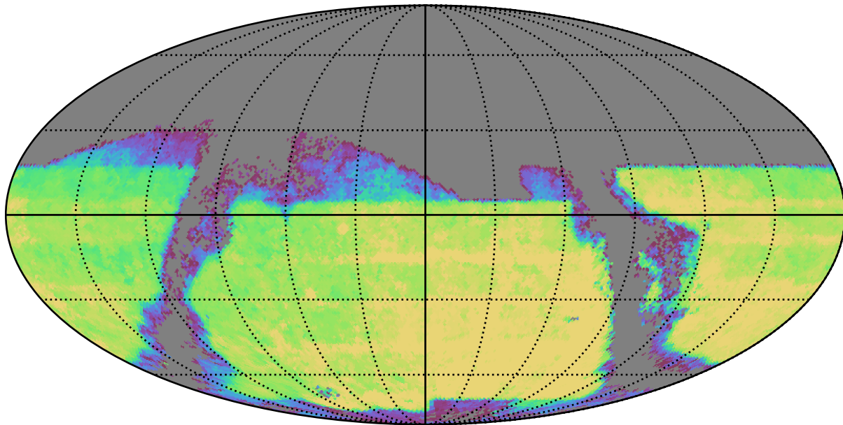
baseline_v2.0_10yrs : TDC_season
