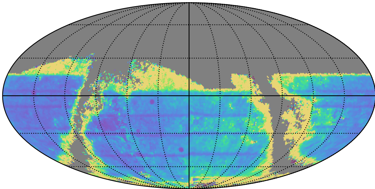
baseline_v2.0_10yrs : TDC_cadence
