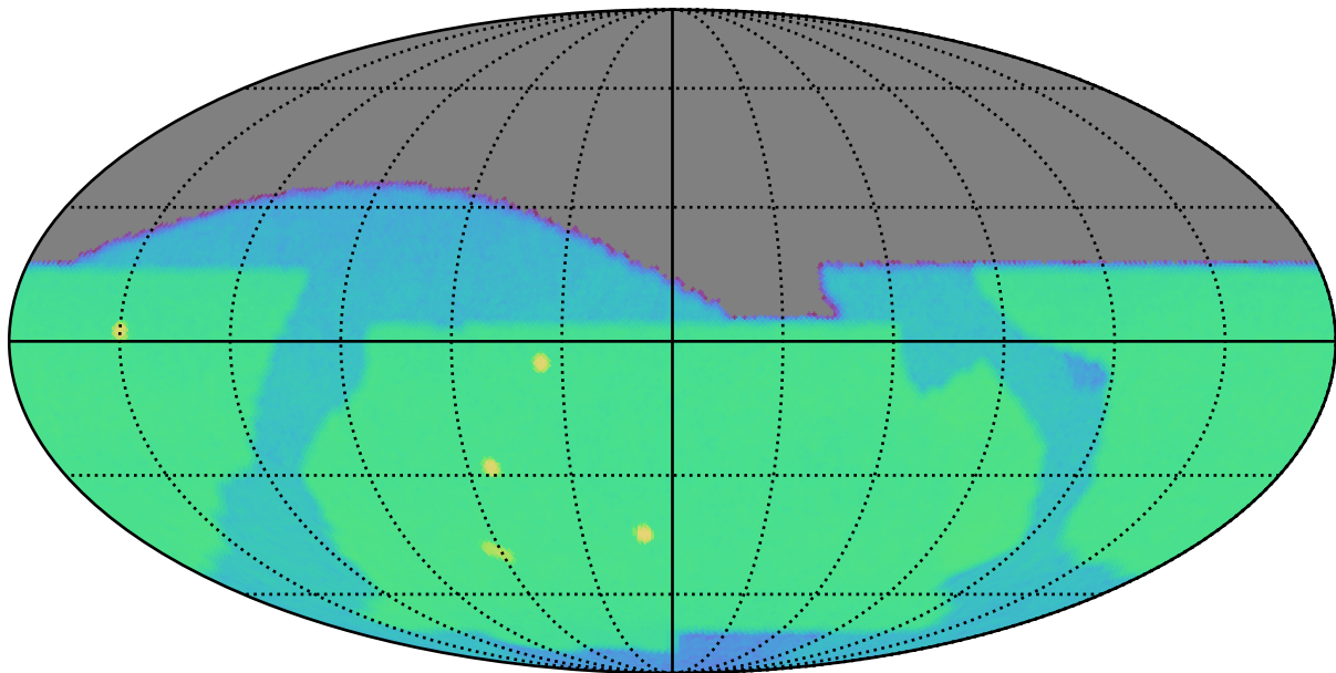
baseline_v2.0_10yrs z: SurfaceBrightLimit
