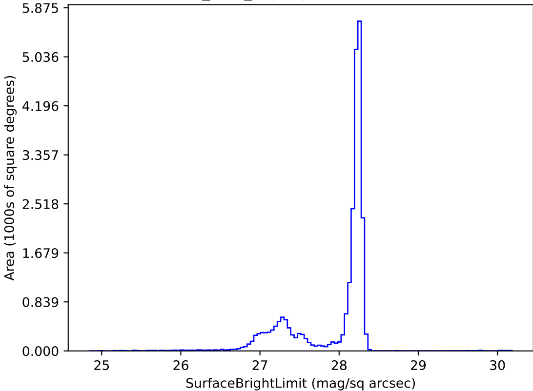
baseline_v2.0_10yrs y: SurfaceBrightLimit
