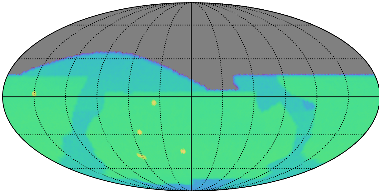
baseline_v2.0_10yrs r: SurfaceBrightLimit
