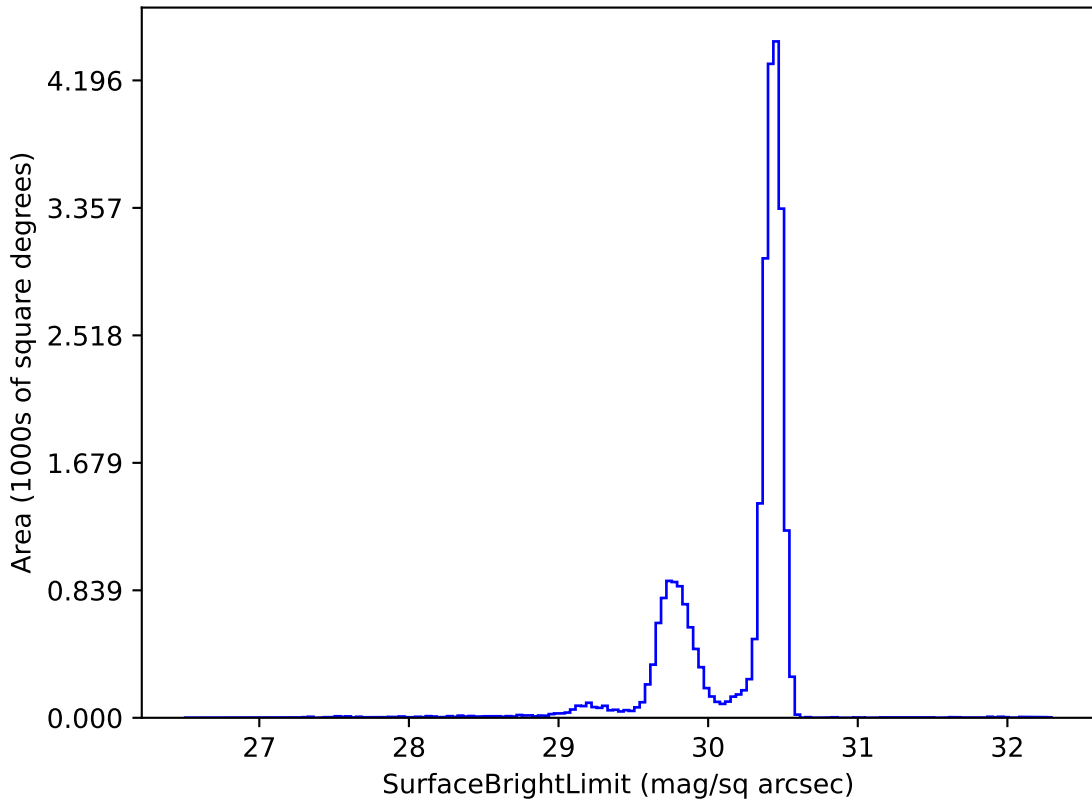
baseline_v2.0_10yrs r: SurfaceBrightLimit
