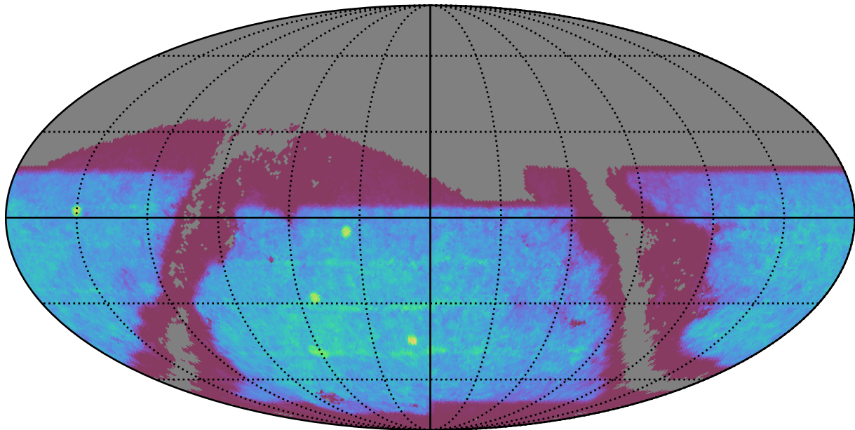
baseline_v2.0_10yrs : SNSLMetric
