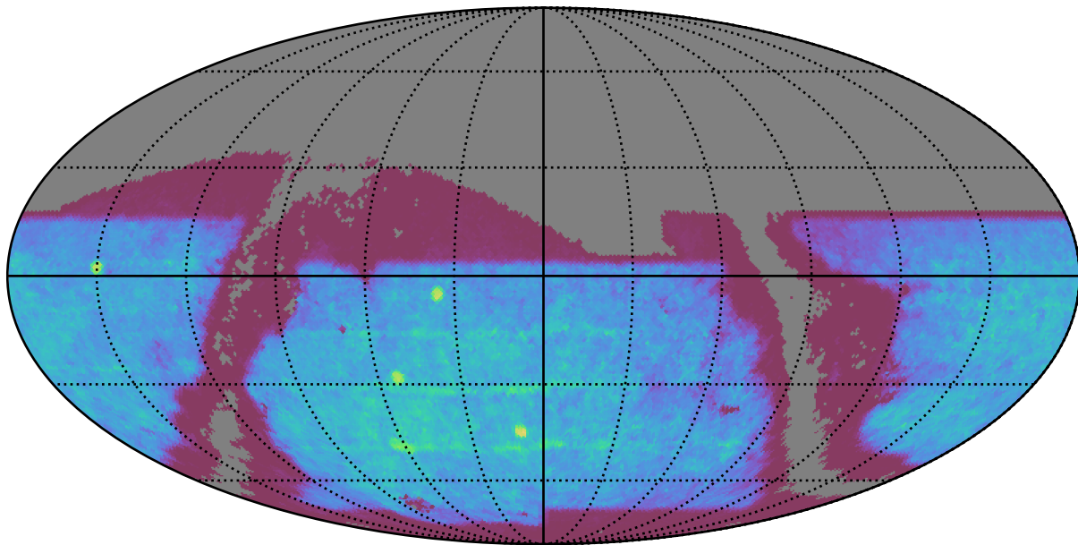
baseline_v2.0_10yrs : SNSLMetric
