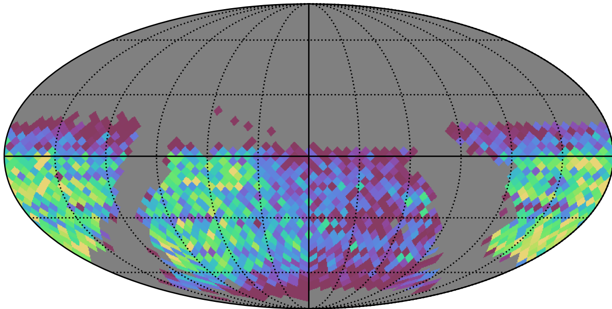
baseline_v2.0_10yrs DDF excluded: SNNSNMetric_reducezlim
