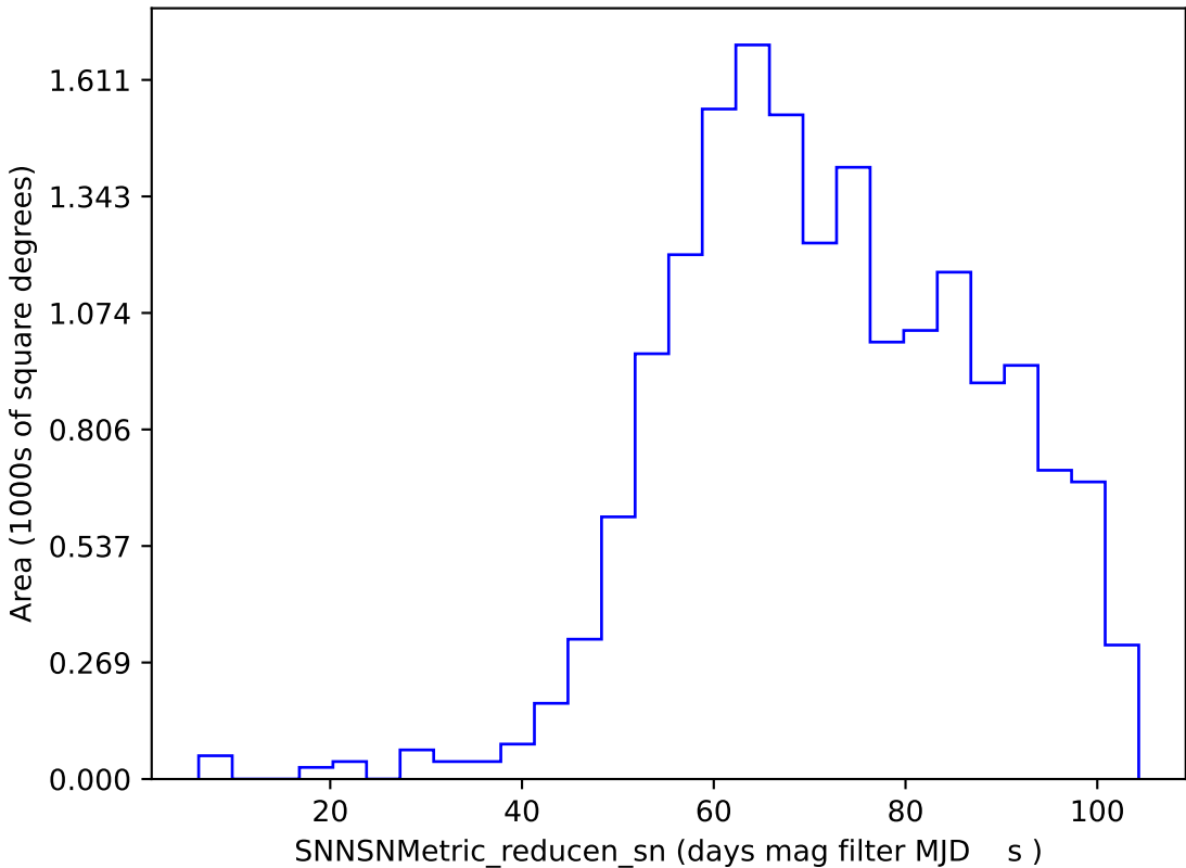
baseline_v2.0_10yrs DDF excluded: SNNSNMetric_reducen_sn
