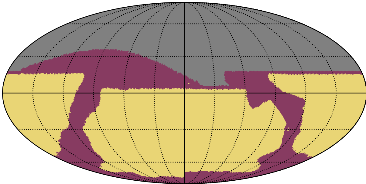
baseline_v2.0_10yrs : RapidRevisits
