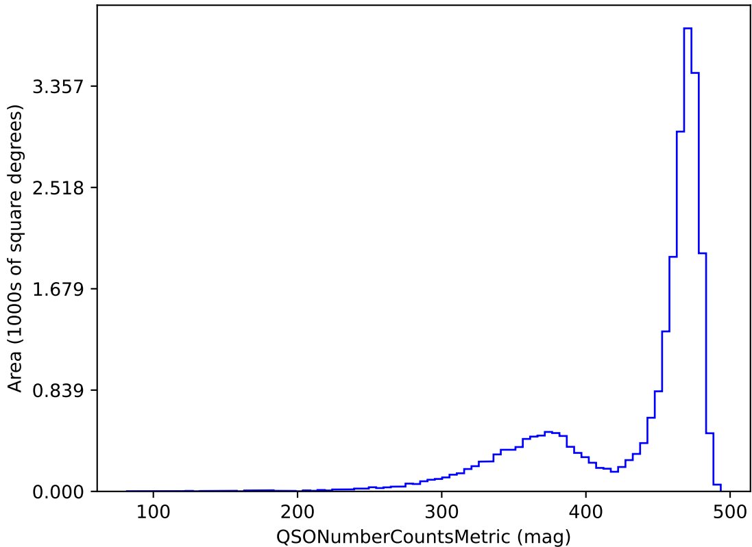
baseline_v2.0_10yrs z band and non-DD: QSONumberCountsMetric
