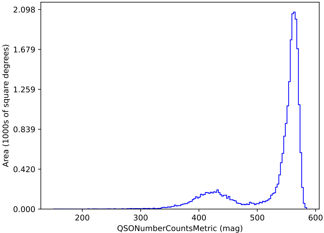
baseline_v2.0_10yrs y band and non-DD: QSONumberCountsMetric
