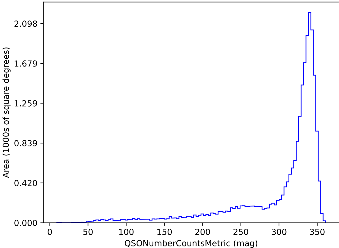
baseline_v2.0_10yrs u band and non-DD: QSONumberCountsMetric
