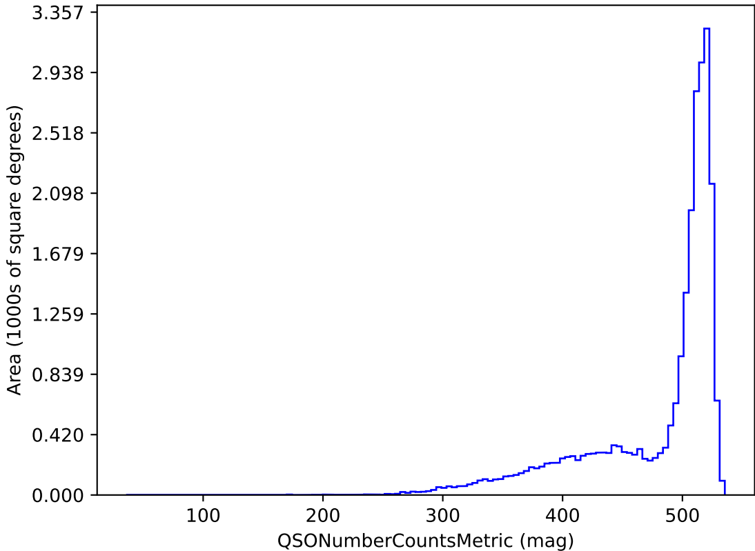
baseline_v2.0_10yrs r band and non-DD: QSONumberCountsMetric
