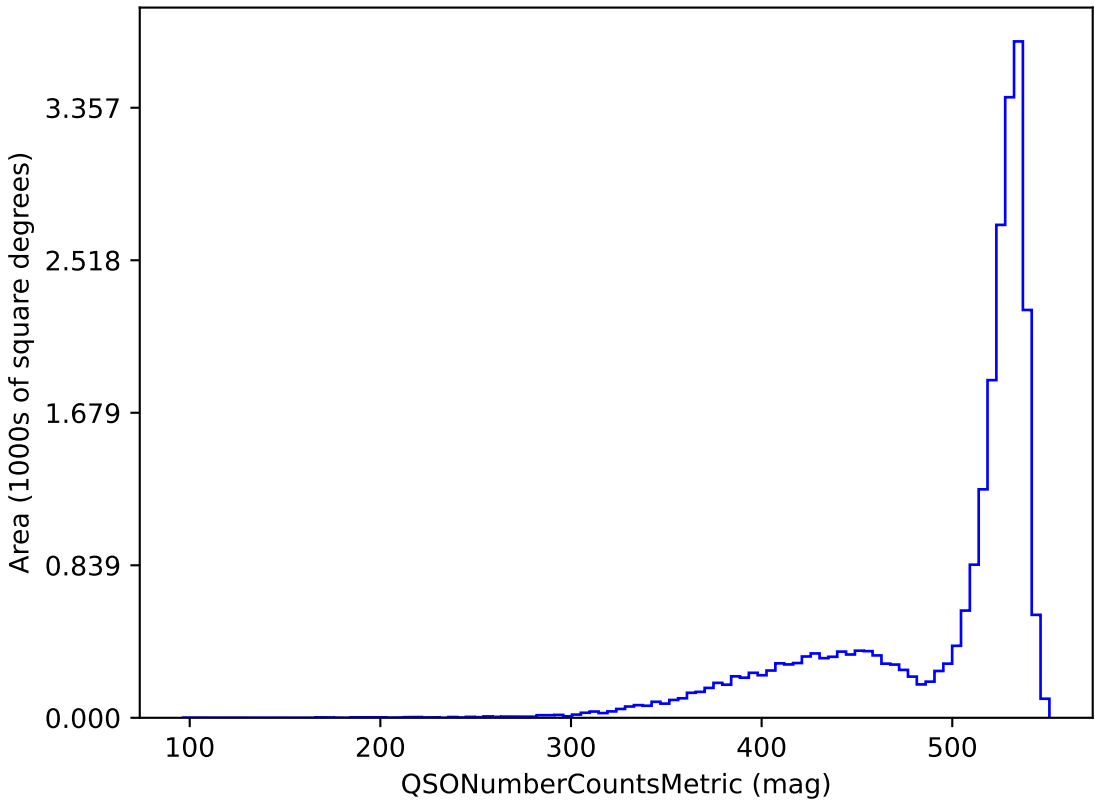
baseline_v2.0_10yrs i band and non-DD: QSONumberCountsMetric
