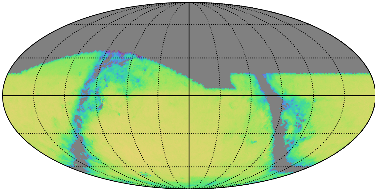
baseline_v2.0_10yrs g band and non-DD: QSONumberCountsMetric
