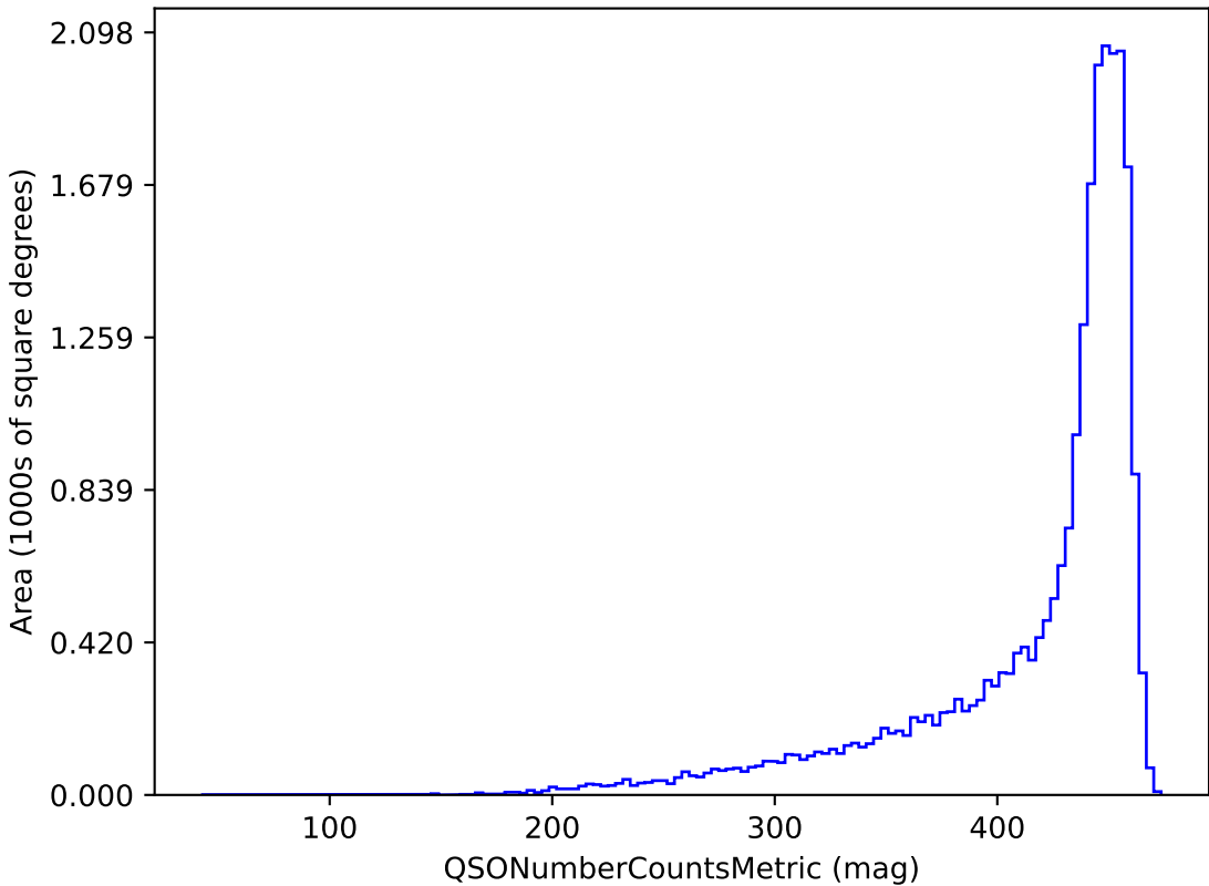
baseline_v2.0_10yrs g band and non-DD: QSONumberCountsMetric
