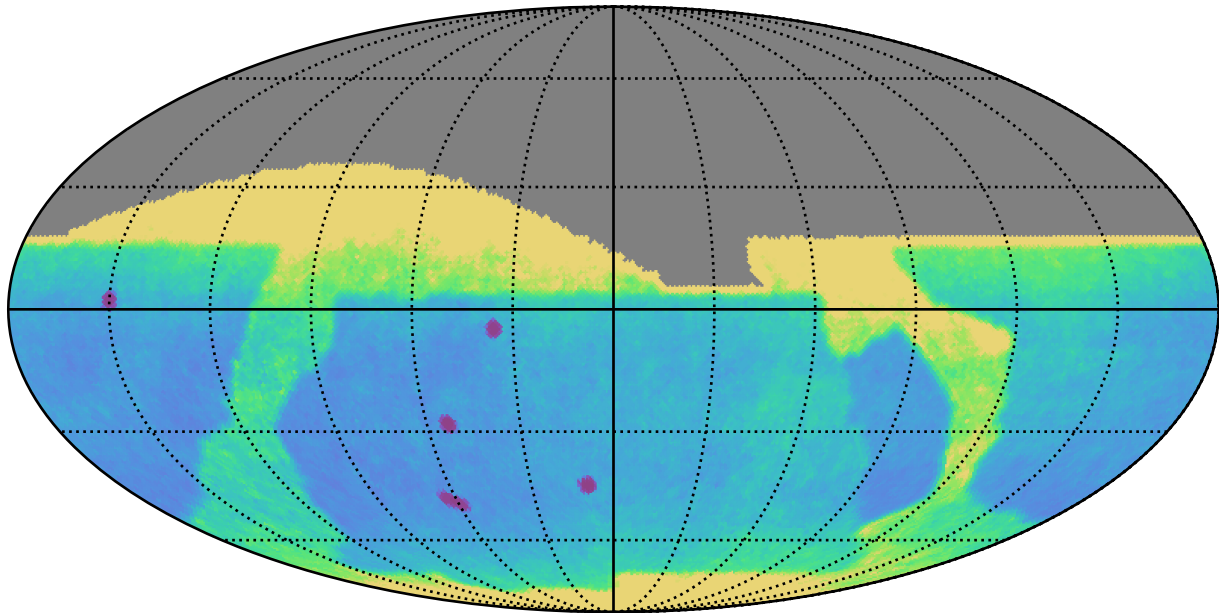
baseline_v2.0_10yrs : Proper Motion Uncert @ 24.0
