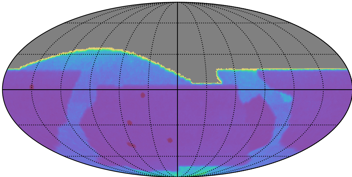
baseline_v2.0_10yrs : Proper Motion Uncert @ 20.5
