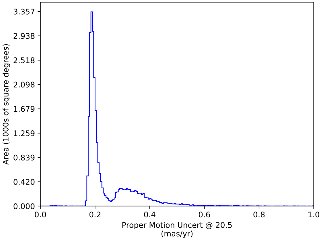
baseline_v2.0_10yrs : Proper Motion Uncert @ 20.5
