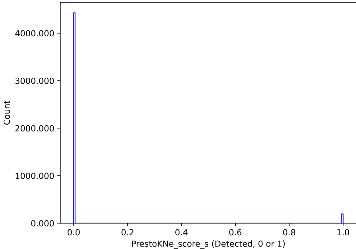
baseline_v2.0_10yrs : PrestoKNe_score_s
