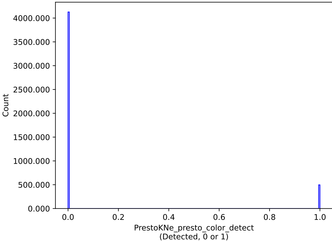
baseline_v2.0_10yrs : PrestoKNe_presto_color_detect
