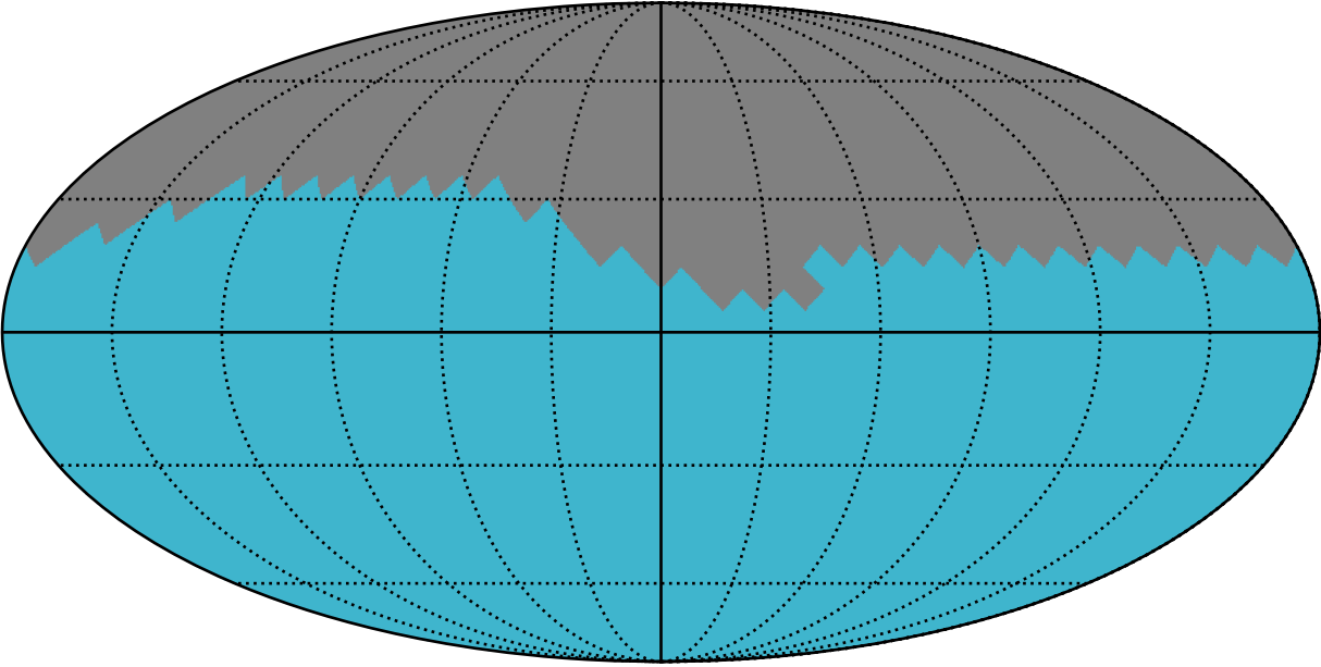
baseline_v2.0_10yrs dm 21 interval 15 RRC Year 1-2: PeriodicStarModulationMetric
