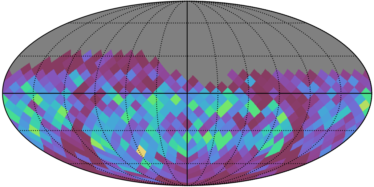
baseline_v2.0_10yrs dm 20 interval 15 RRC Year 1-2: PeriodicStarModulationMetric
