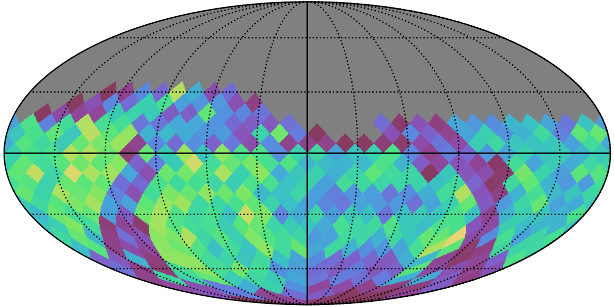
baseline_v2.0_10yrs dm 18 interval 30 RRc Year 1-2: PeriodicStarModulationMetric
