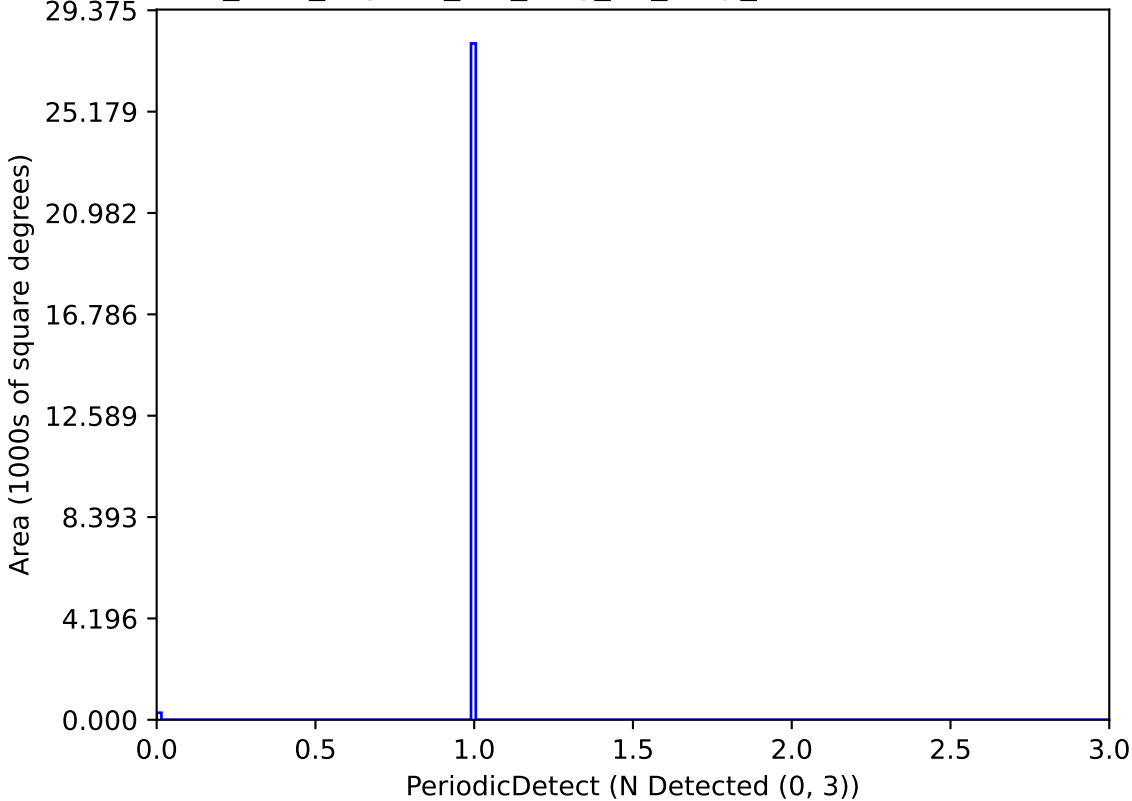
baseline_v2.0_10yrs P_2.0_Mag_24_Amp_0.05-0.1-1: PeriodicDetect
