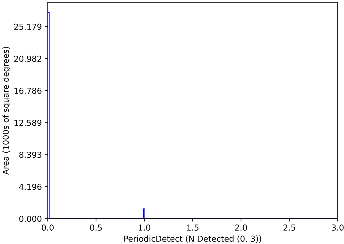
baseline_v2.0_10yrs P_1.0_Mag_24_Amp_0.05-0.1-1: PeriodicDetect
