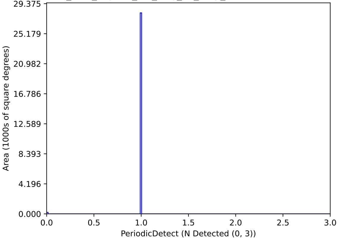
baseline_v2.0_10yrs P_0.5_Mag_24_Amp_0.05-0.1-1: PeriodicDetect
