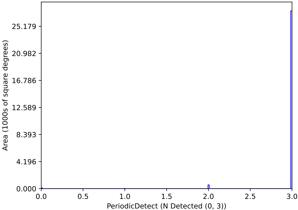
baseline_v2.0_10yrs P_0.5_Mag_21_Amp_0.05-0.1-1: PeriodicDetect
