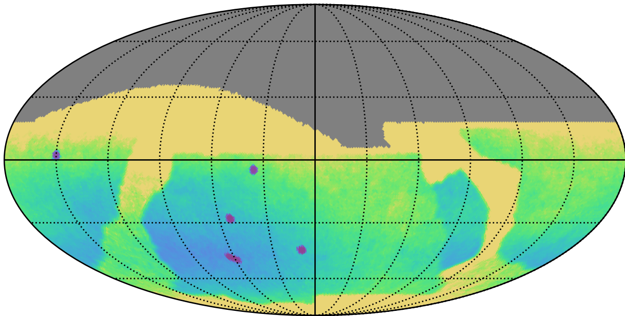
baseline_v2.0_10yrs : Parallax Uncert @ 24.0
