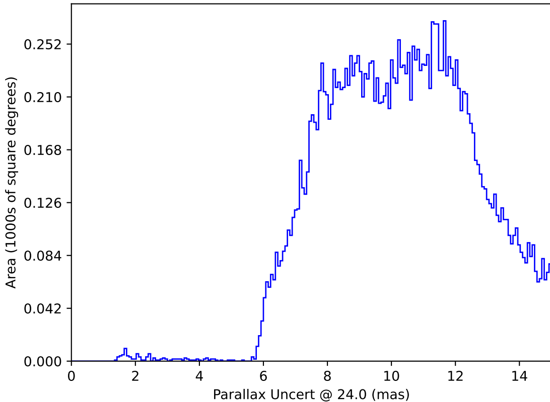
baseline_v2.0_10yrs : Parallax Uncert @ 24.0
