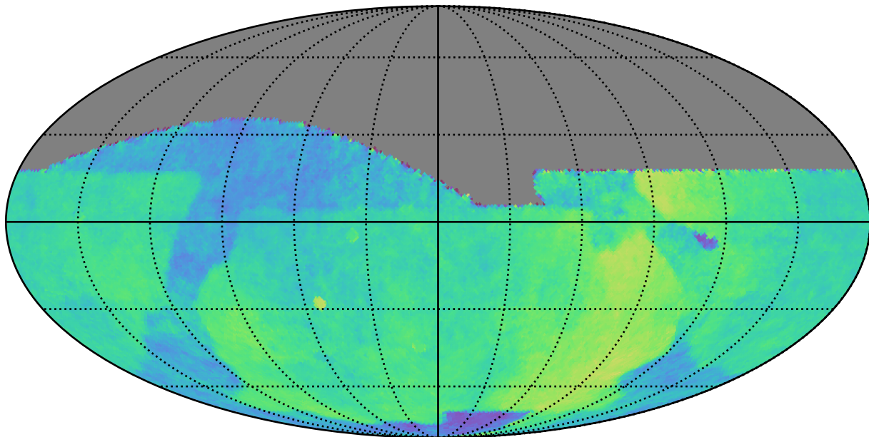
baseline_v2.0_10yrs : Parallax Coverage @ 24.0
