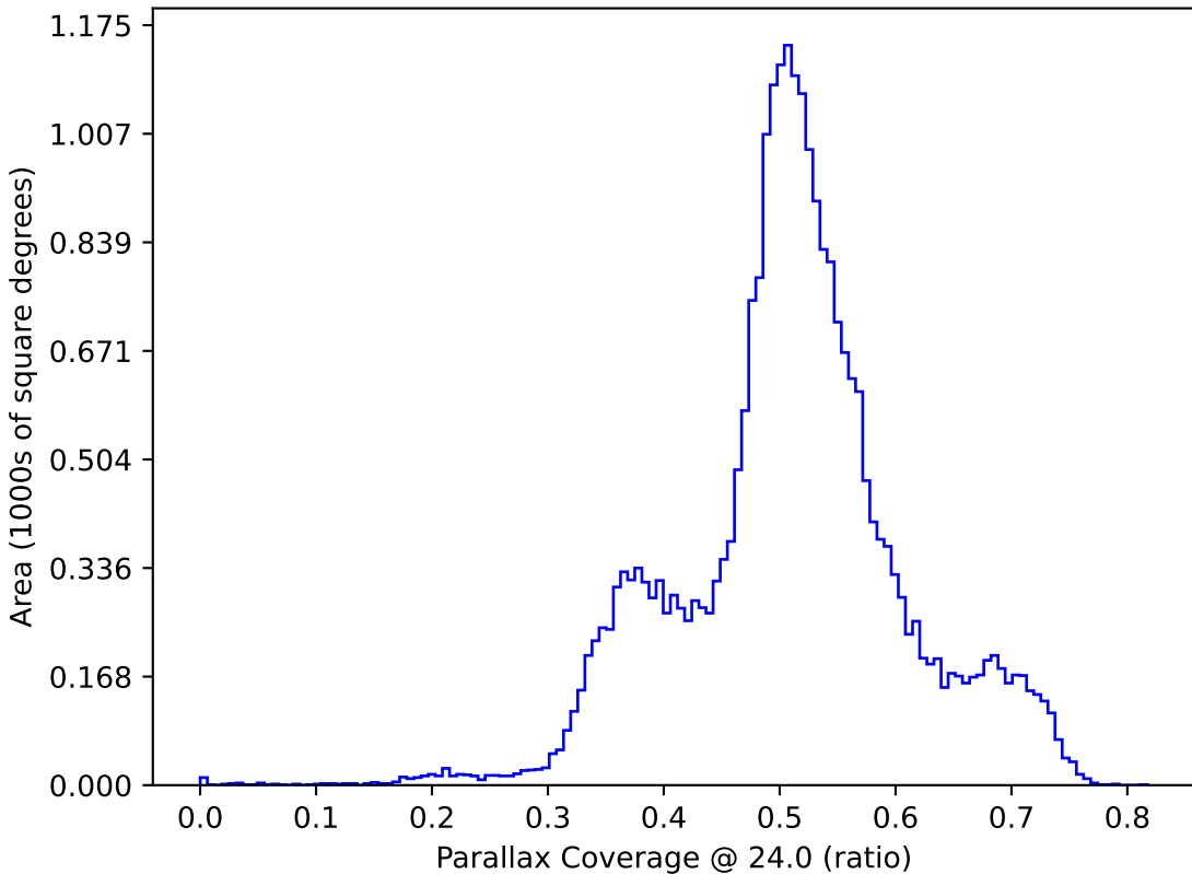
baseline_v2.0_10yrs : Parallax Coverage @ 24.0
