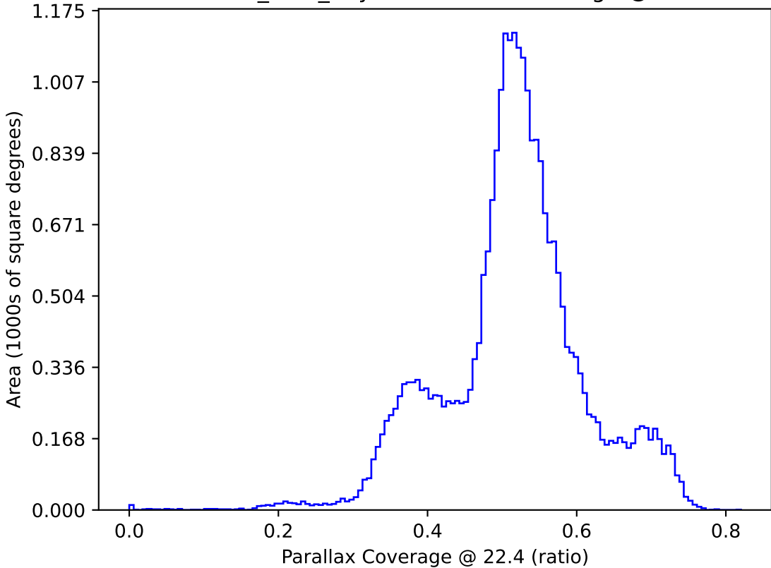
baseline_v2.0_10yrs : Parallax Coverage @ 22.4
