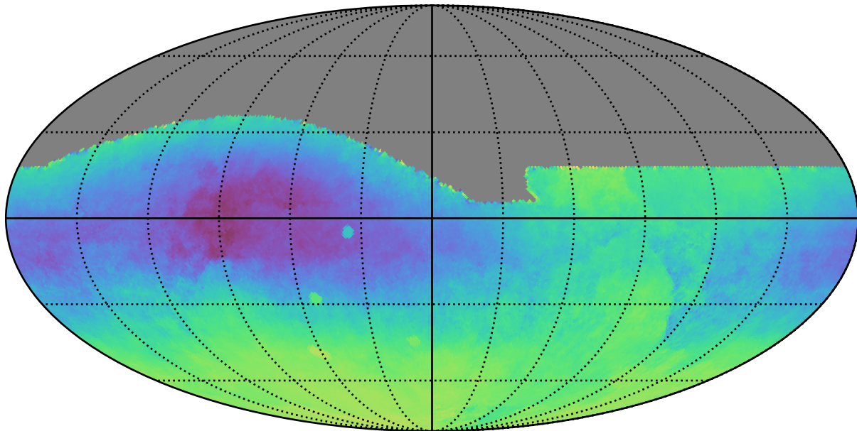
baseline_v2.0_10yrs : Parallax-DCR degeneracy @ 24.0
