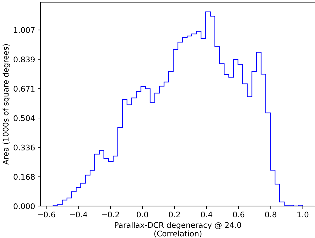
baseline_v2.0_10yrs : Parallax-DCR degeneracy @ 24.0
