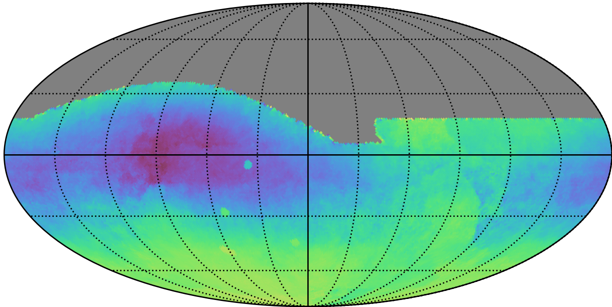
baseline_v2.0_10yrs : Parallax-DCR degeneracy @ 22.4
