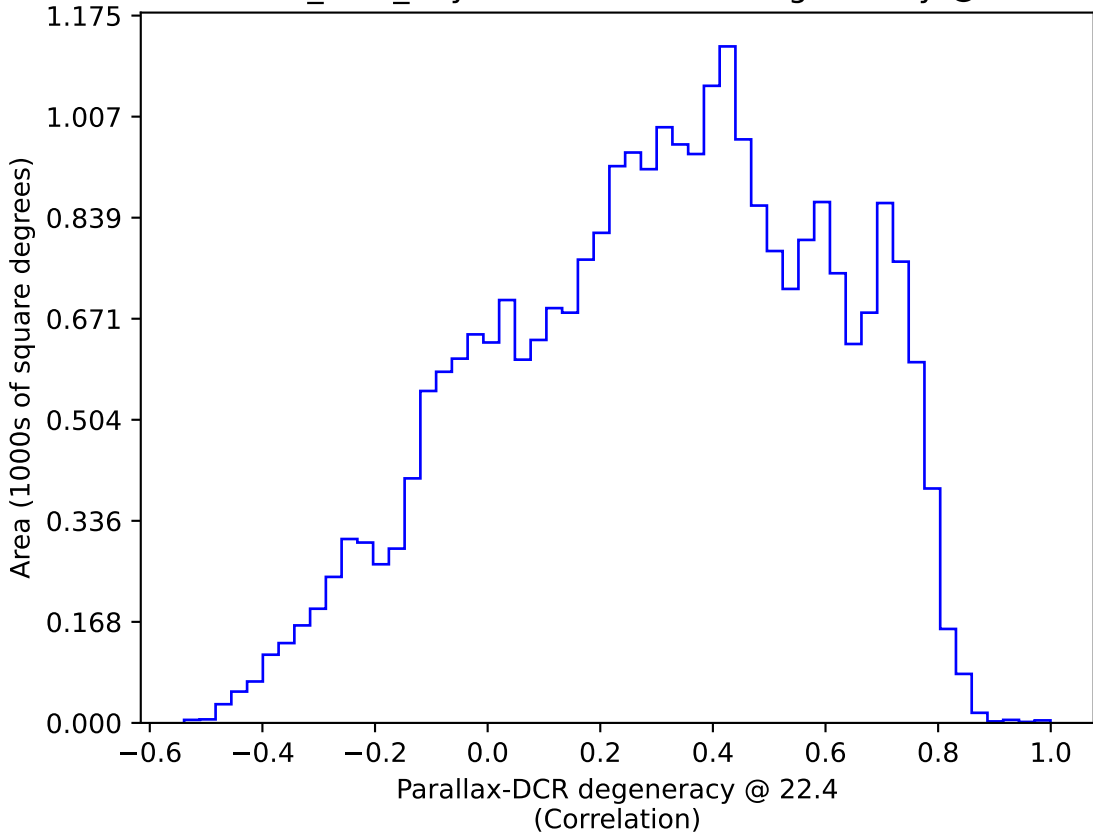
baseline_v2.0_10yrs : Parallax-DCR degeneracy @ 22.4
