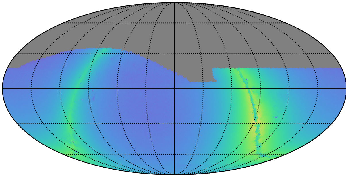
baseline_v2.0_10yrs z: Nstars_no_crowding
