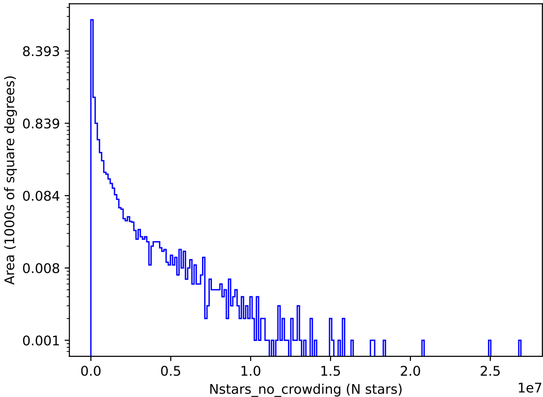
baseline_v2.0_10yrs z: Nstars_no_crowding
