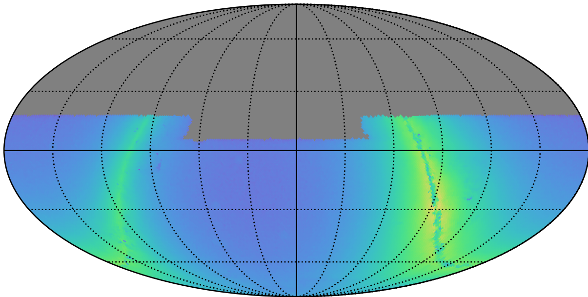
baseline_v2.0_10yrs y: Nstars_no_crowding
